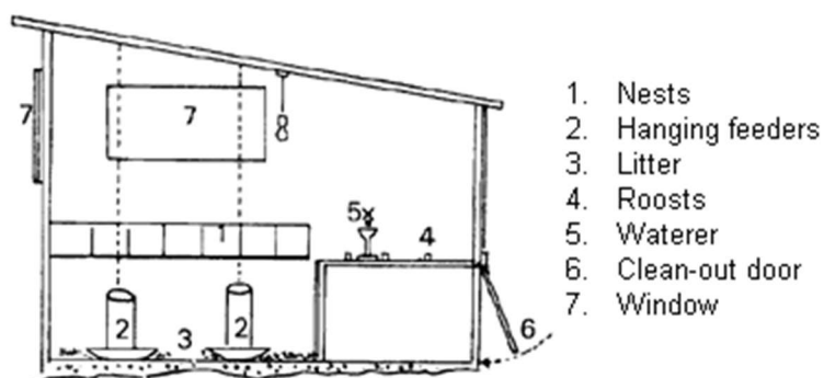
Figure 2. Side view of house contents
